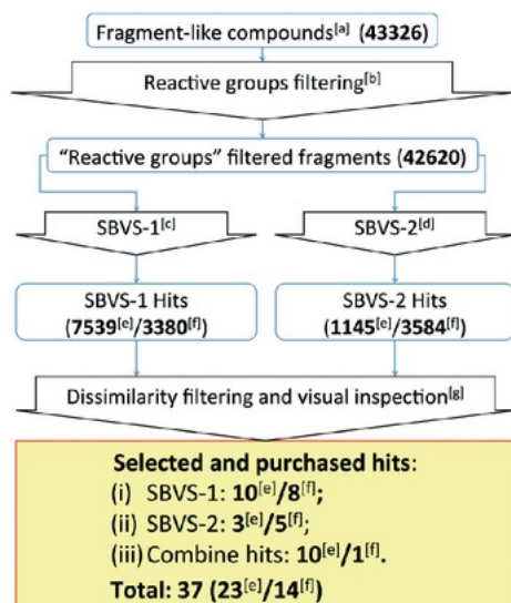
Fig. 5 Flowchart of the \beta_2 R-based and H_4 R-based prospective SBVS campaigns. See Experimental section for more details. [a] Fragment-like compounds collected from the ZINC database. 37,99 [b] Filtering fragments containing plausible reactive/toxic groups. 100 [c] SBVS with JNJ777120 (2) as the reference compound. 7,56,80 [d] SBVS with VUF10497 (3) as the reference compound. 8,56,63 [e] Results from the \beta_2 R-based prospective SBVS studies. [f] Results from the H_4 R-based prospective SBVS studies. [g] Fragments with ECFP-4 Tanimoto similarity score of less than 0.40 to any of the H_4 R ligands used in the retrospective VS. 24 In the H_4 R-based prospective SBVS campaigns, H_4 R purchased hits from the \beta_2 R-based prospective SBVS studies were added as the reference compounds in the dissimilarity filtering.
