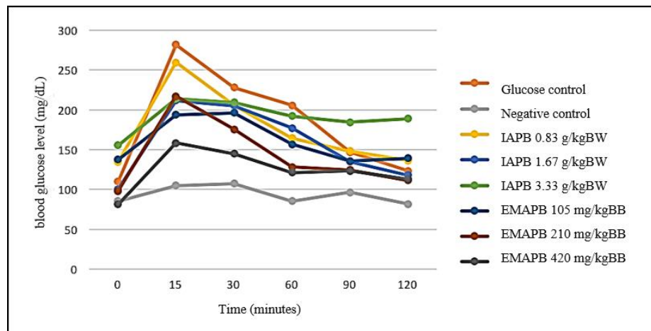
Figure 1. Correlation curve between time and the blood glucose level average in the pasak bumi roots infusion treatment (IAPB) and pasak bumi roots methanol extract (EMAPB)
