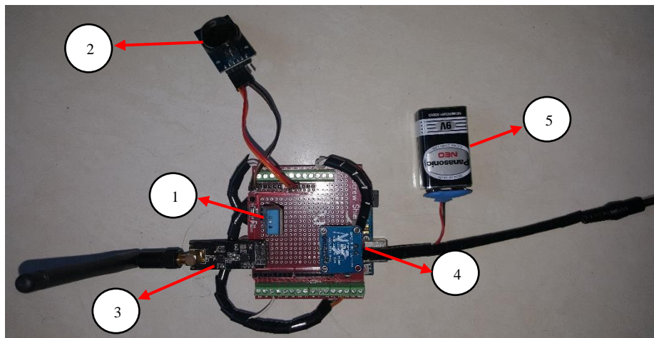
Gambar 3.2 Modul Node Sensor
