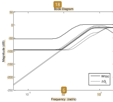
Figure 6. Complimentary sensitivity weight Wt and the system uncertainty of the base joint control
