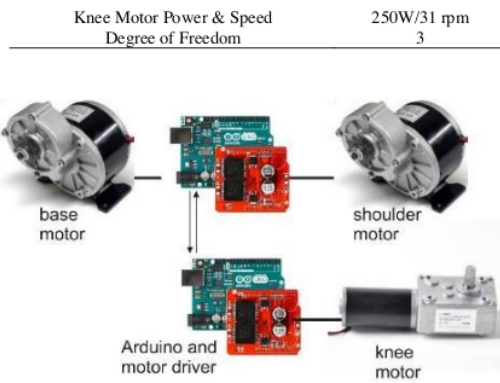
Figure 2. Controller connection of the robotic arm
