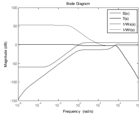
Figure 6. The sensitivity, complementary sensitivity, and their inverse weight singular values of the base joint
