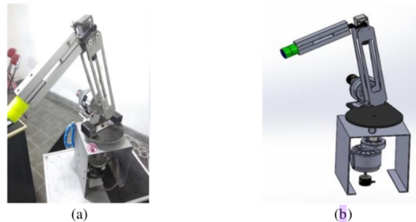
Figure 1. (a) Robotic arm prototype; (b) Mechanical design of 3DoF articulated robotic arm
