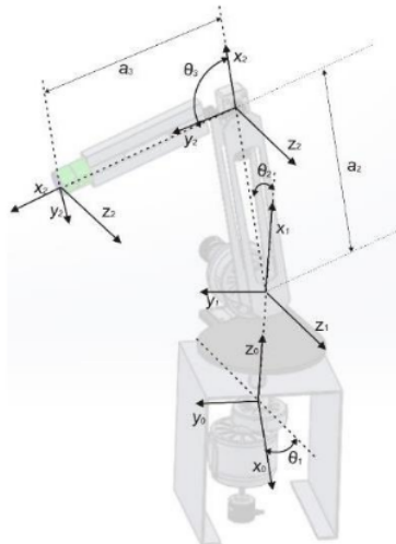
Figure 3. Reference coordinate systems on the robotic arm
