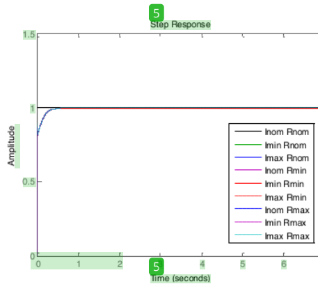
Figure 8. System response using proposed controller
