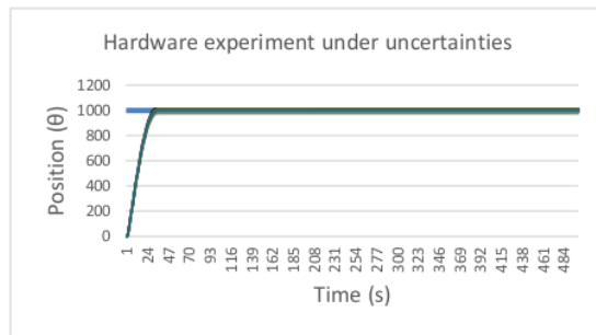
Figure 12. Hardware response system using the proposed controller
