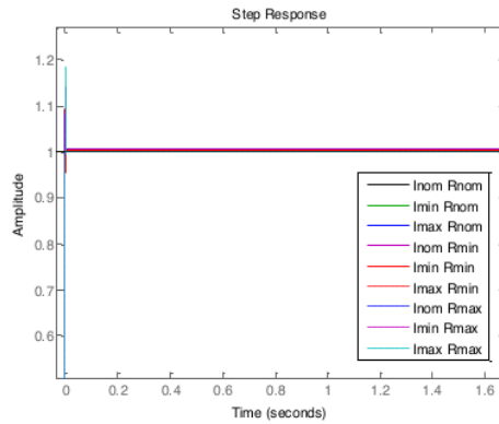
Figure 11. System response using auto tuned PID controller
