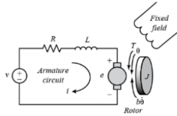
Figure 4. DC motor electrical and mechanical diagram
