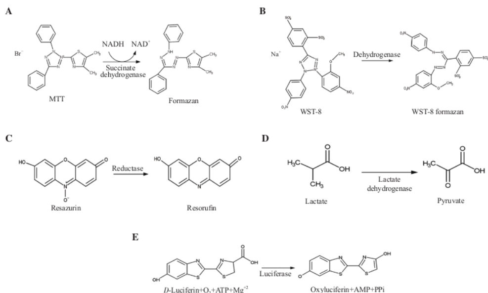
Figure 1. (A) Conversion reaction of 3-(4,5-dimethylthiazol-2-yl)-2,5-diphenyltetrazolium bromide (MTT) to formazan. (B) Conversion of 2-(2-methoxy-4-nitrophenyl)-3-(4-nitrophenyl)-5-(2,4-disulfophenyl)-2H-tetrazolium (WST-8) to the formazan salt. (C) Conversion of resazurin to resorufin. (D) Reduction of lactate to pyruvate. (E) Luciferin oxidation to oxyluciferin. ATP: adenosine 5'-triphosphate; AMP: adenosine monophosphate. The structures are drawn using MarvinSketch.
