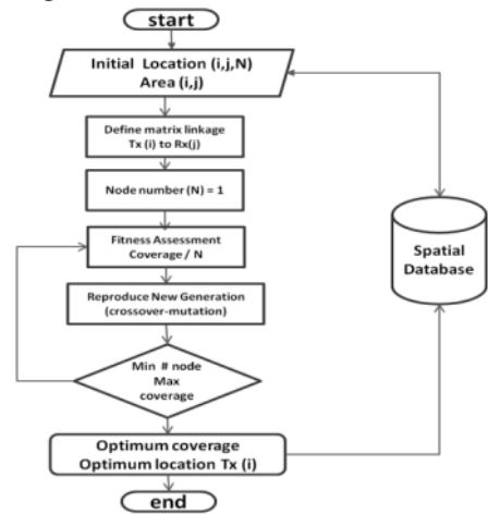
Figure 11. Optimization Flowchart
