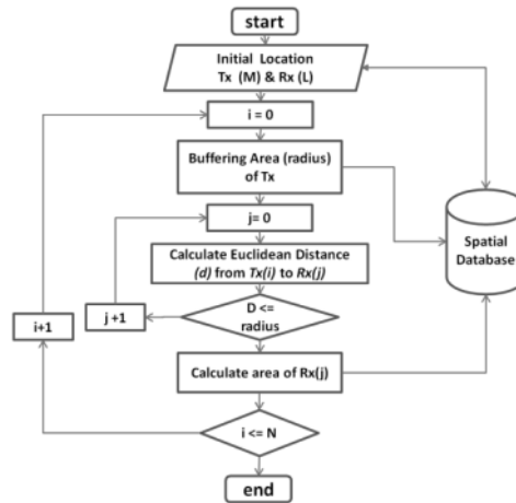
Figure 8. GIS Model for Interconnection and Distance between APs and RPs
