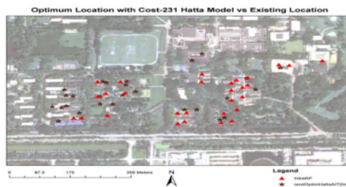
Figure 14. Optimum Access Point Location
