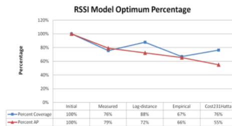
Figure 13. RSSI Model Comparison of Optimization
