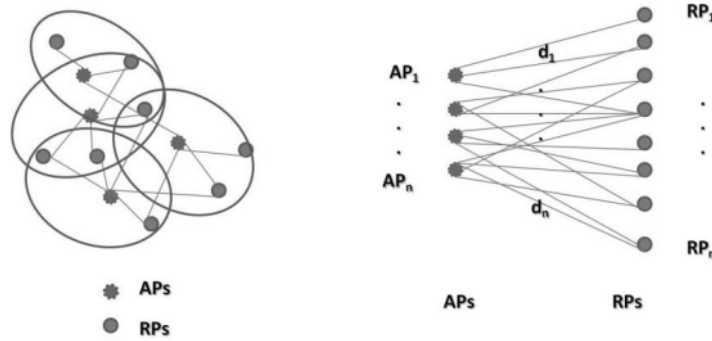
Figure 4. Island-based Algorithm Model for Optimization of AP Placement
