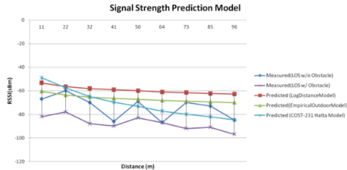
Figure 9. Comparison of Measured and Predicted Signal
