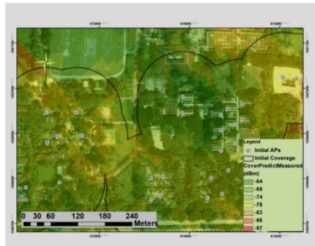
Figure 10. Initial Coverage Signal Strength in the Study Area
