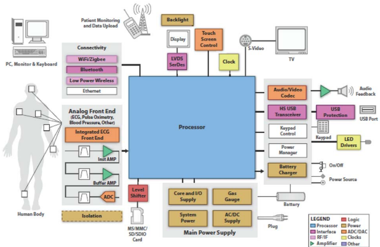
Gambar 2. Diagram Blok Patient Monitor (Texas Instrument, 2010)
