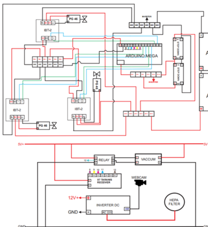
Figure 4. Robot Wirings
