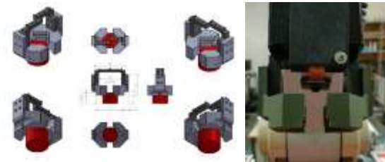
Figure 8. Redesign of gripper
