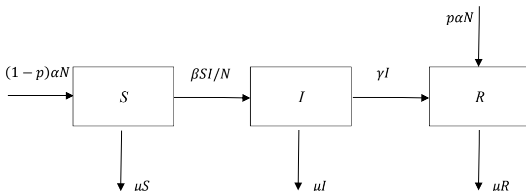
GAMBAR 1. Diagram Alir Model Epidemiologi SIR
