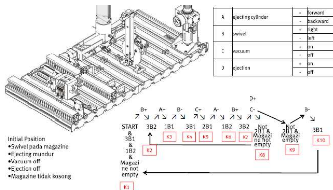
Figure 5. Sequential Diagram.
