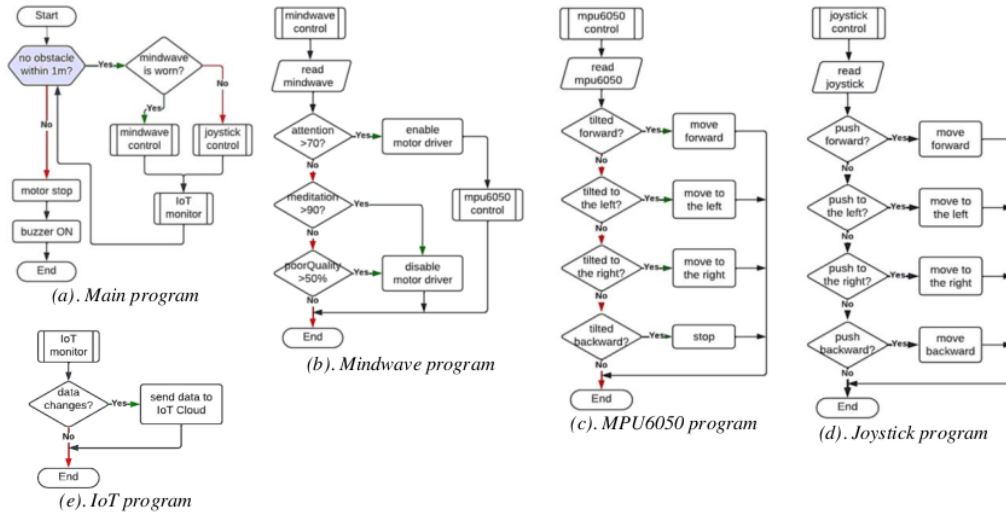
Figure 3. Flowchart of: (a). main program; (b). mindwave program; (c). MPU6050 program; (d). joystick program; and (e). IoT program
