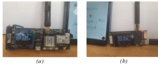
Figure 6. (a). T-BEAM and (b). TTGO LORA ESP32
