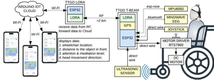
Figure 2. Block diagram of the wheelchair control system
