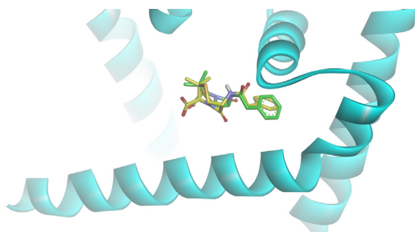
Figure 4. The superimposition of the initial (yellow) and re-docked (green) pose in the active site of TcaR (PDB ID 3KP2).
