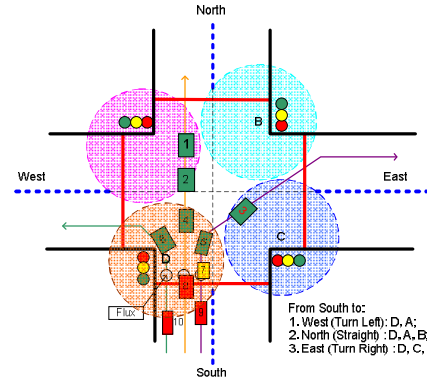
Figure 4: The architecture of the RFID-based red light violation detection
