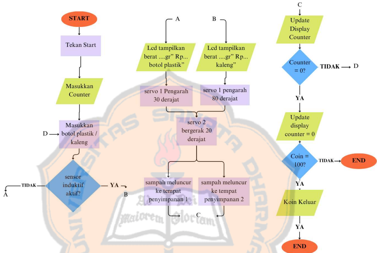
Gambar 3. 6 Flowchart Sistem Trash2Cash
