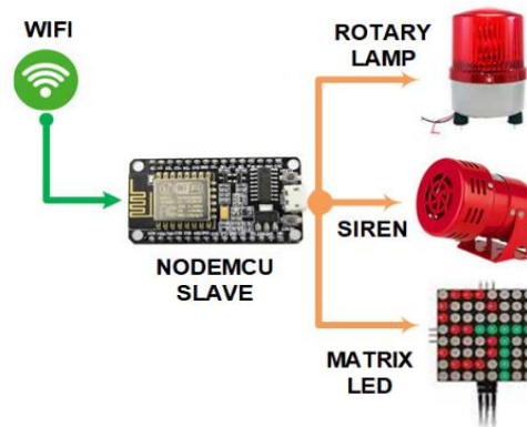
Figure 3. The wiring diagram of the slave unit
