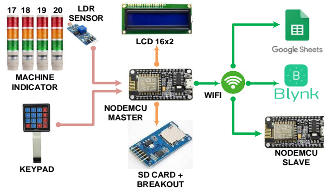
Figure 2. The wiring diagram of the master unit
